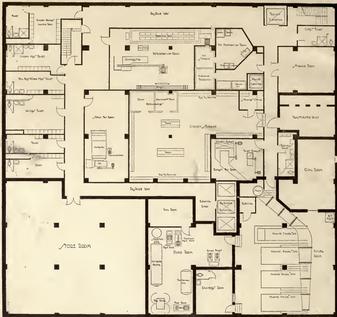
BASEMENT PLAN
